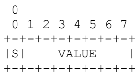
Figure B.1.3 -- Song Select Command Log Format
