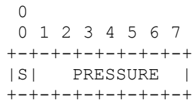
Figure A.8.1 -- Chapter T Format
