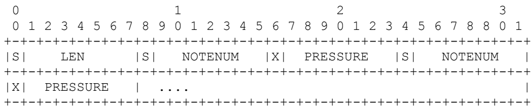
Figure A.9.1 -- Chapter A Format
