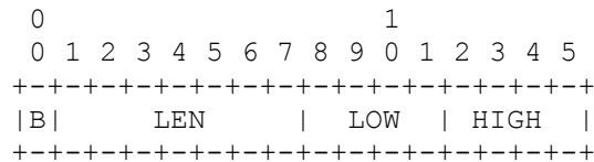
Figure A.6.2 -- Chapter N Header
