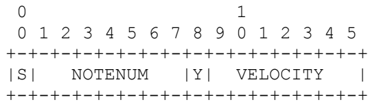
Figure A.6.3 -- Chapter N Note Log
