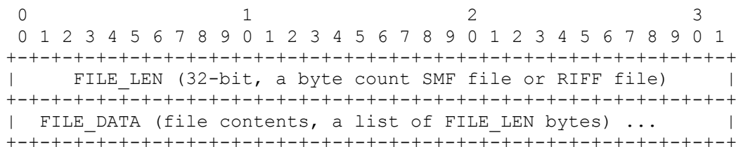
Figure E.5 -- The FILE_BLK Field Format
