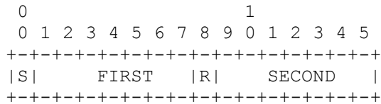
Figure A.5.1 -- Chapter W Format
