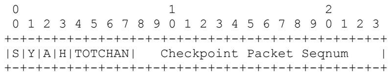
Figure 7 -- Top-Level Recovery Journal Format
