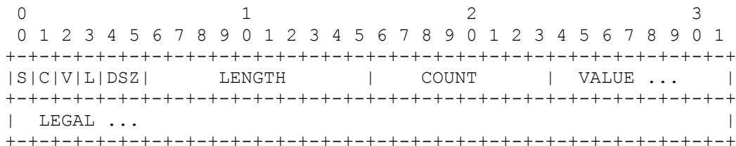
Figure B.1.4 -- Undefined System Common Command Log Format
