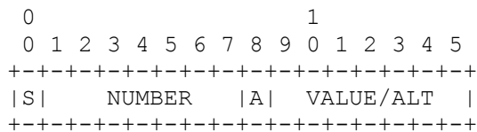
Figure A.3.2 -- Chapter C Controller Log
