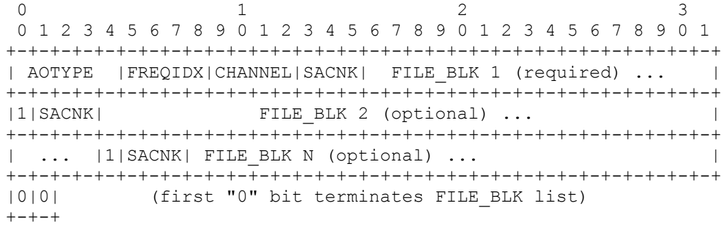
Figure E.3 -- Simplified AudioSpecificConfig
