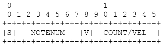
Figure A.7.2 -- Chapter E Note Log
