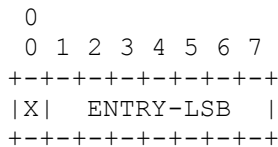
Figure A.4.4 -- ENTRY-LSB Field
