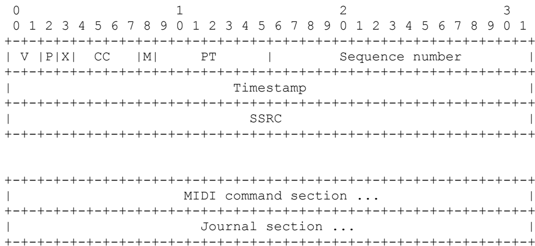
Figure 1 -- Packet Format
