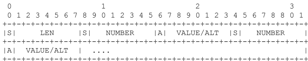
Figure A.3.1 -- Chapter C Format
